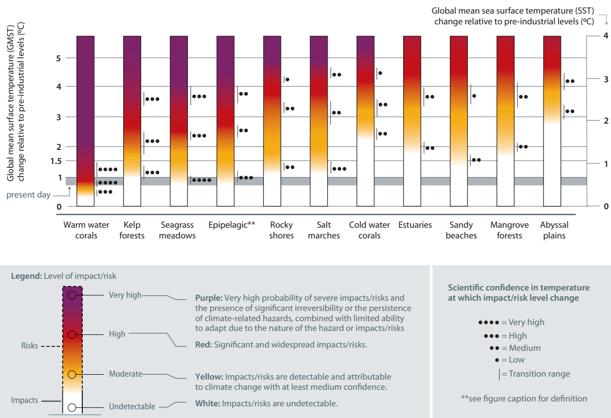
Figure 2: Every degree of global warming will harm coastal ecosystems further 22
