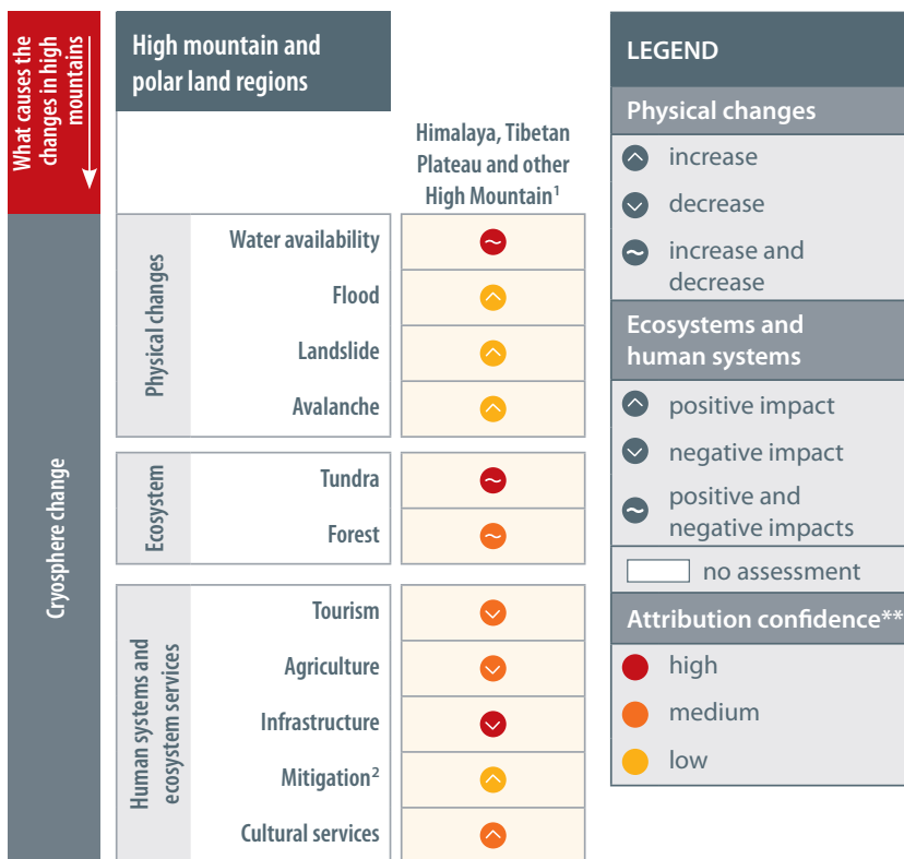
Figure 4: How changes in the atmosphere and the climate have affected the cryosphere 60
