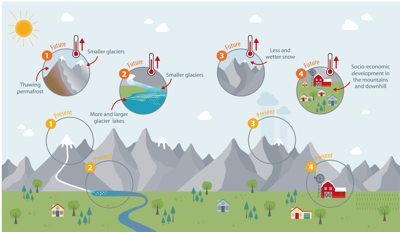
Figure 6: Anticipated changes in high mountain hazards as the climate changes 73
