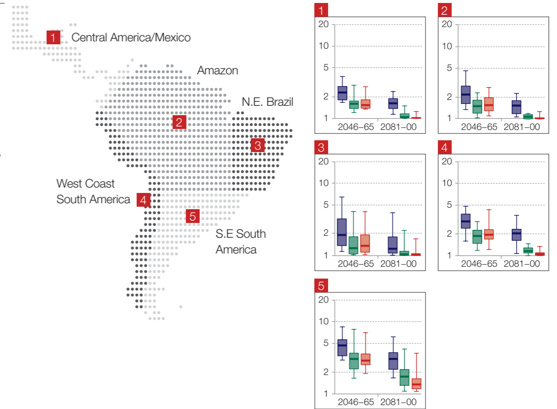
Figure 2: Projected return period (in years) of late 20th century 20-year return values of annual maximum (a) of the daily maximum temperature; and (b) 24-hour precipitation rates
