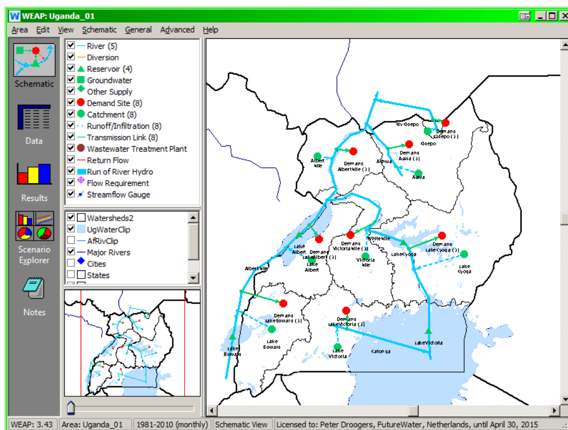
Figure 15. Schematic overview of the WEAP model applied to Uganda.
