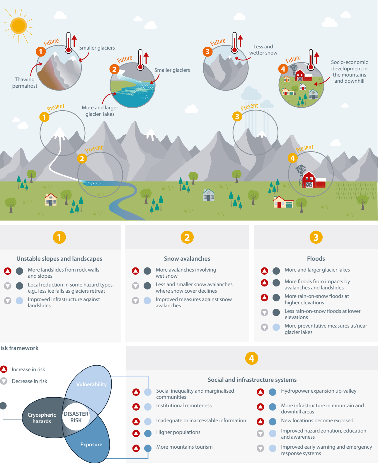
Figure 6: Anticipated changes in high mountain hazards as the climate changes 73
