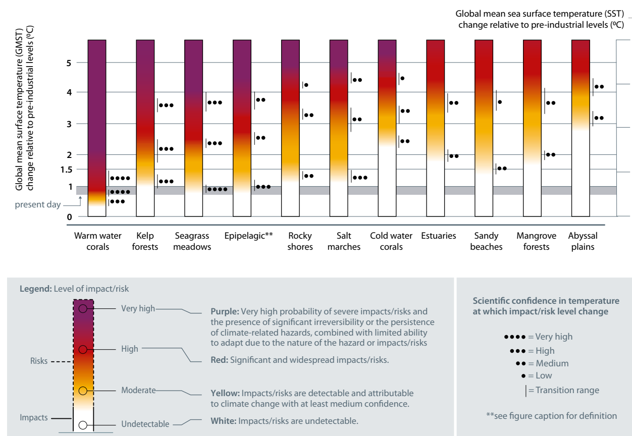
Figure 2: Every degree of global warming will harm coastal ecosystems further 22
